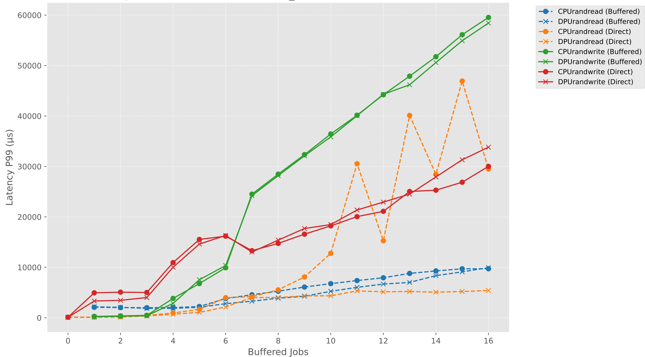
Latency P99 vs Buffered Jobs (direct1_bufferedN) - RAND (CPU vs DPU)
